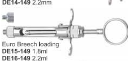
Cartridge Syringe DE13-149 1.8mm DE14-149 2.2mm
